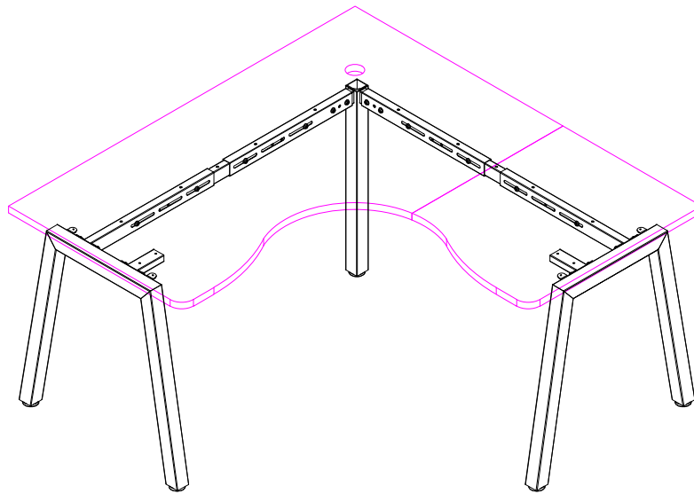
ISOMETRIC
