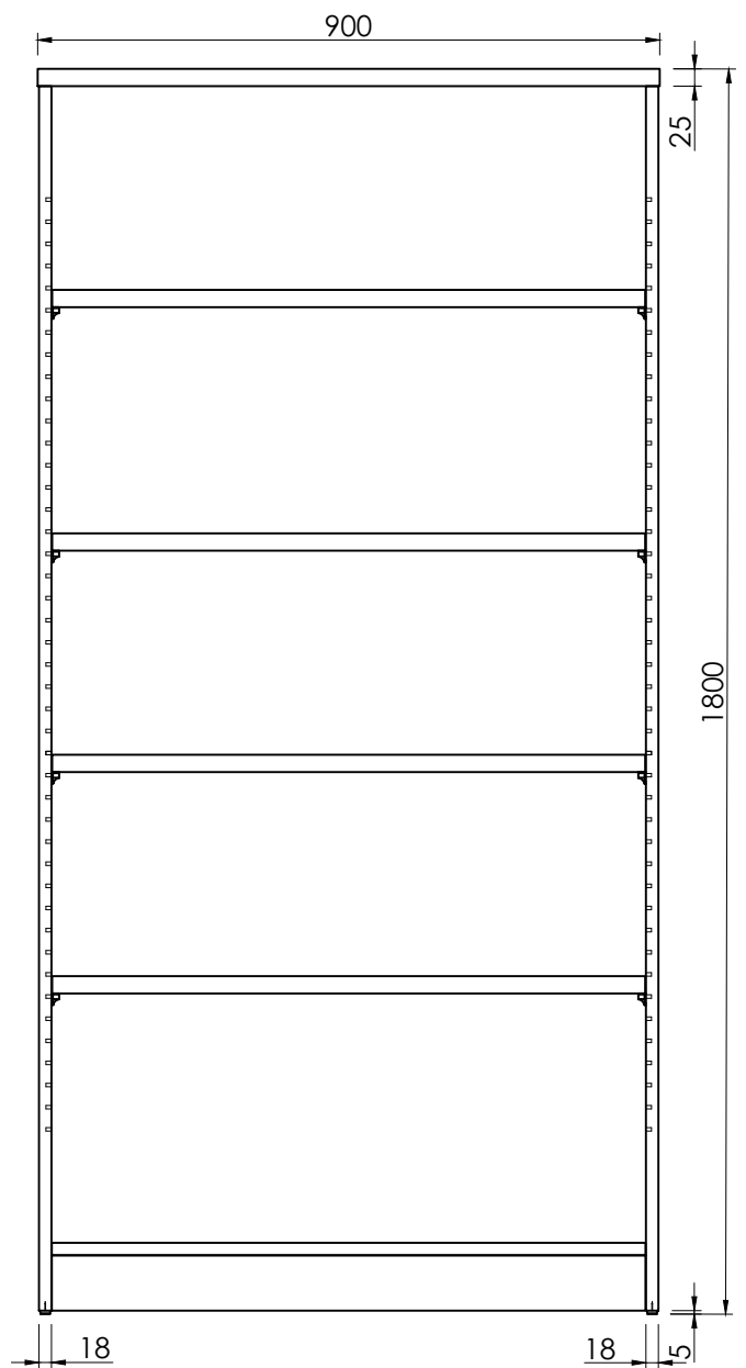
FRONT VIEW
