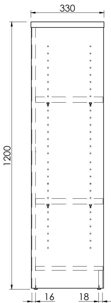
SIDE VIEW
