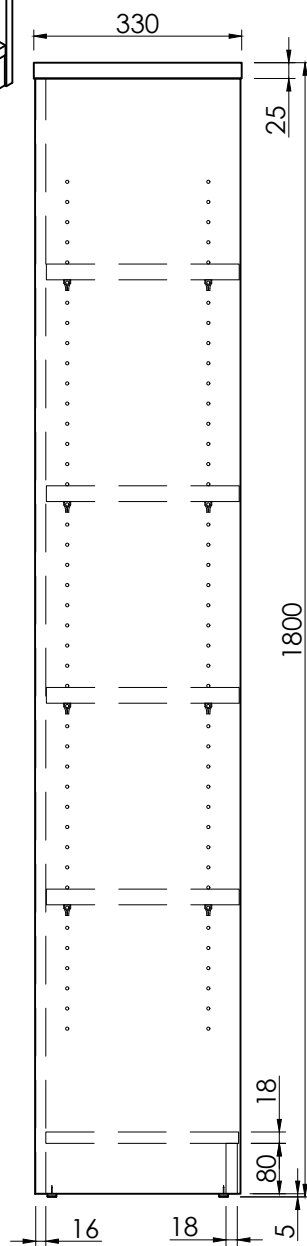
SIDE VIEW
