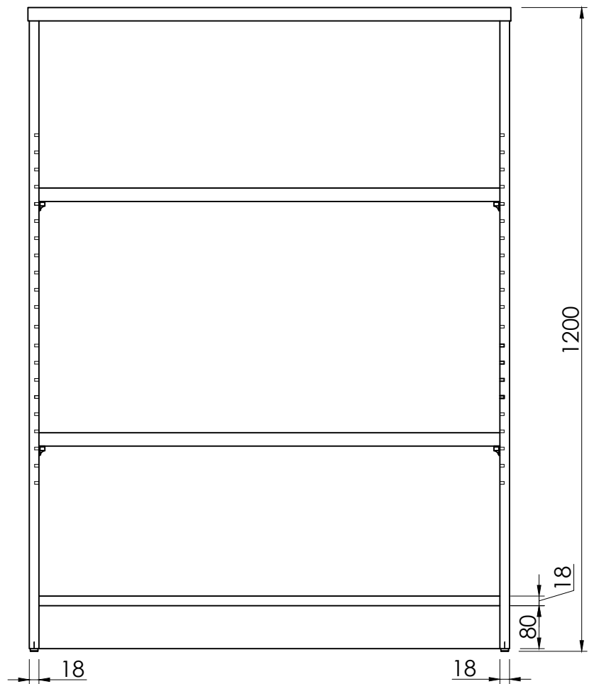
FRONT VIEW
