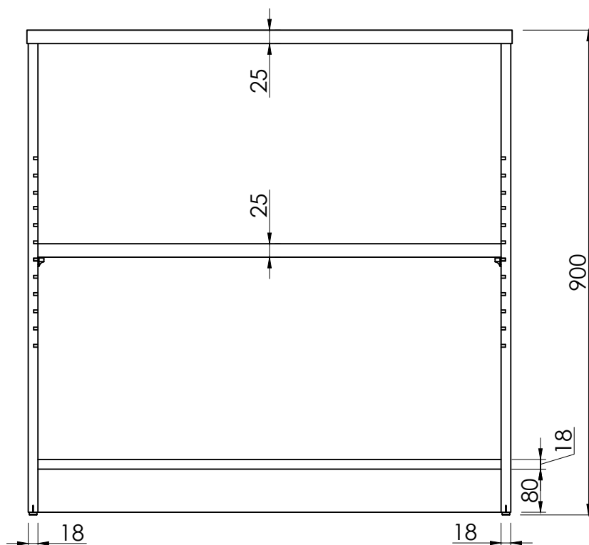
FRONT VIEW
