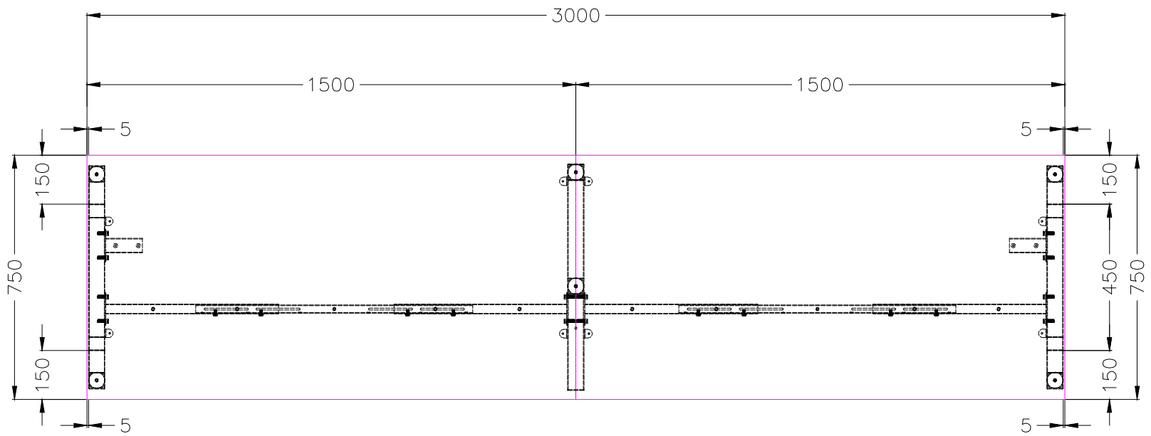
TOP VIEW
