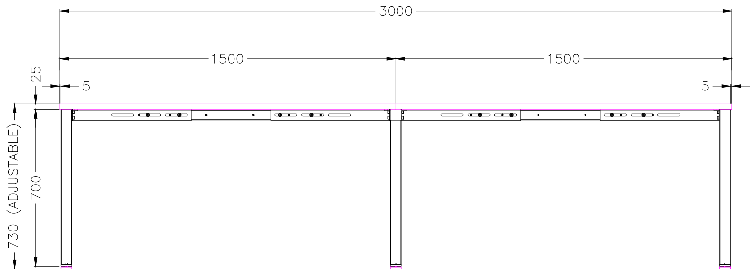
FRONT VIEW
